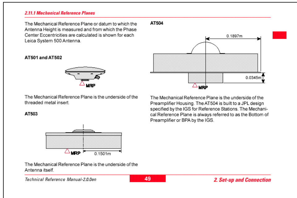
Figure 1 Mechanical Reference Plane for AT502, AT503 & AT504 Antenna Types
