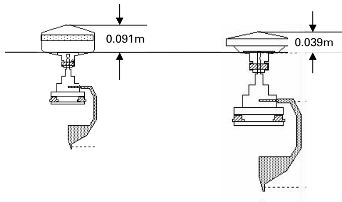
Figure 7 Mechanical Reference Plane for SR299/399 Internal and AT202/302 External Antennas
