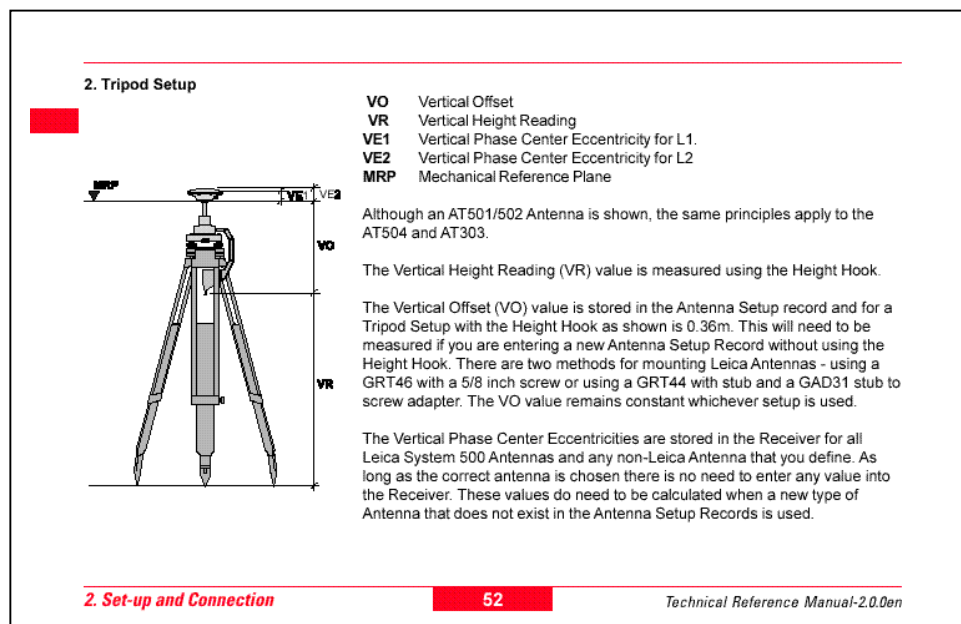
Figure 2 Relationships between Vertical Reading, Offset and Phase Center Locations for an AT503 Antenna Setup on a Tripod
