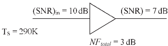
Fig. 2. Noise figure example
