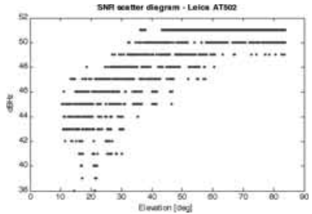
Fig. 7. SNR characteristics of the Leica AT502 antenna.
