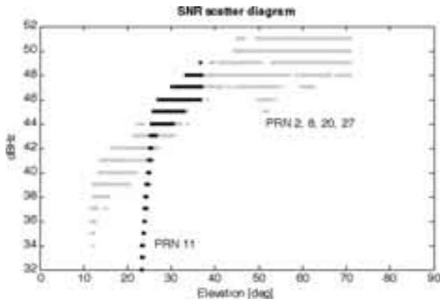
Fig. 11. Example of an abnormal decrease of the signal strength of satellite 11.
