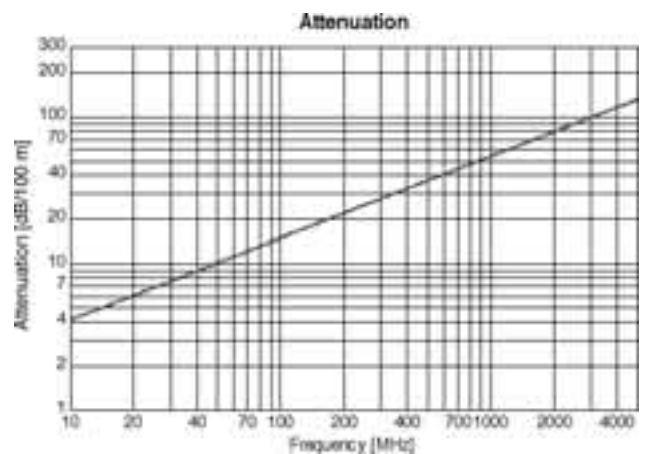
Fig. 4. Attenuation values of a double screened antenna cable (RG 223) at 20°C.
