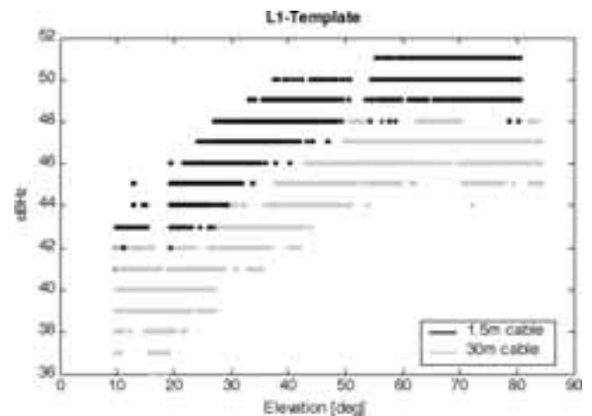
Fig. 5. SNR scatter diagram with a 1.5m antenna cable and with a 30m antenna cable.
